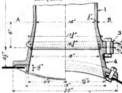
Figs. 461-465. Taper Stack and Brace. Southern Pacific.
